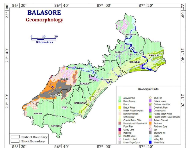
Figure 3: Geomorphology of Balasore District
