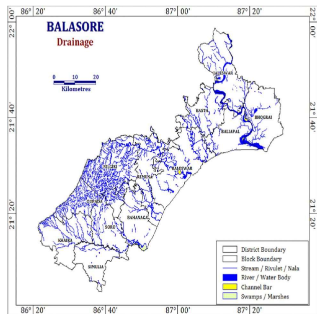
Figure 2: Drainage map of Balasore District.
