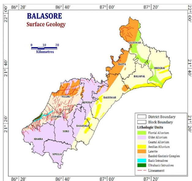
Figure 4: Surface Geological Map of Balasore District
