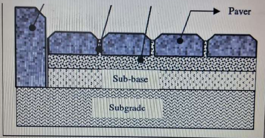
Figure 1. Structure of concrete block pavement
