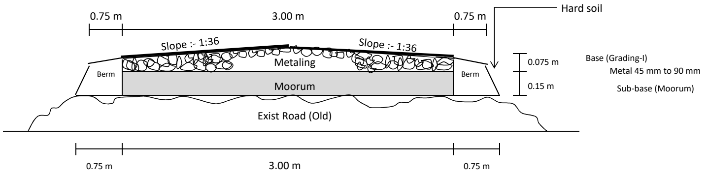
CROSS SECTION OF WBM ROAD
