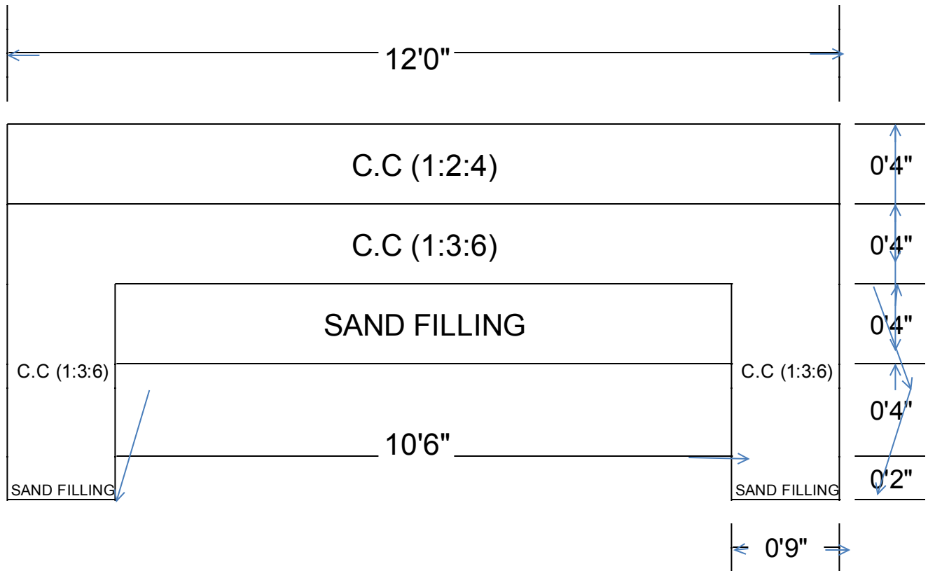
CROSS SECTION OF C.C ROAD
