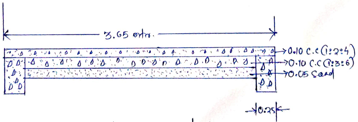
section of a c.e road
