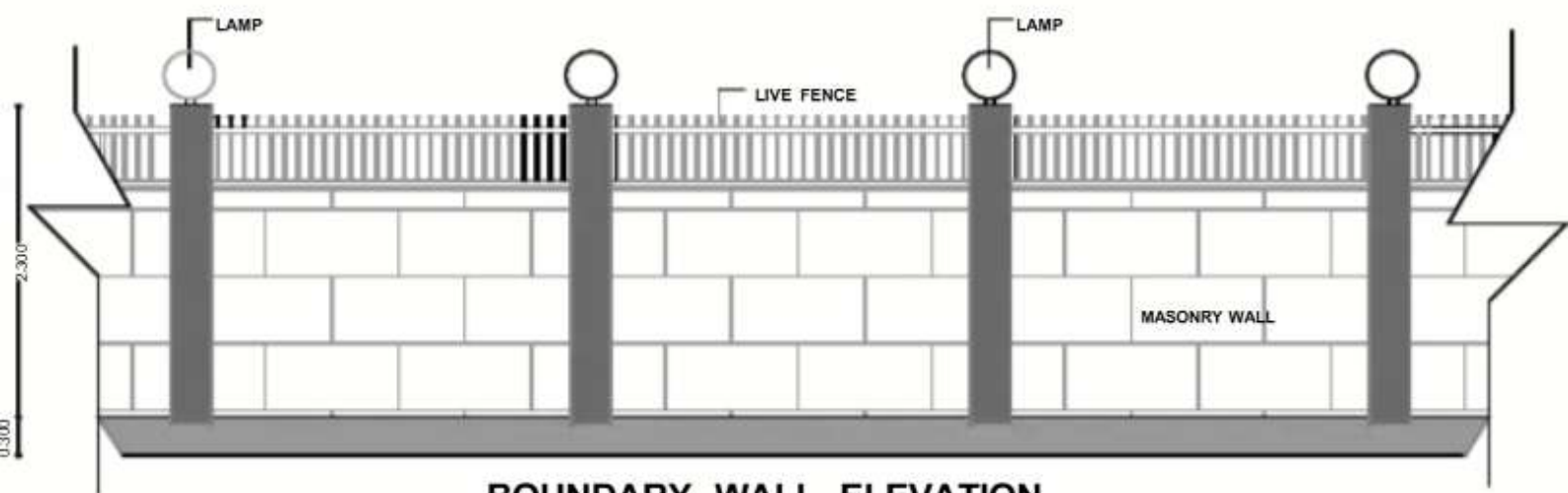
BOUNDARY WALL ELEVATION
