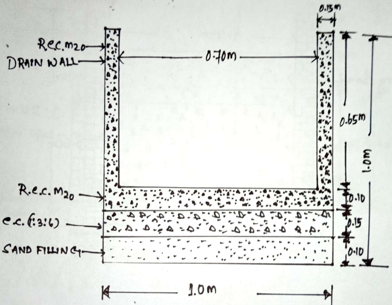
CROSS SECTION OF R.C.C. DRAIN
