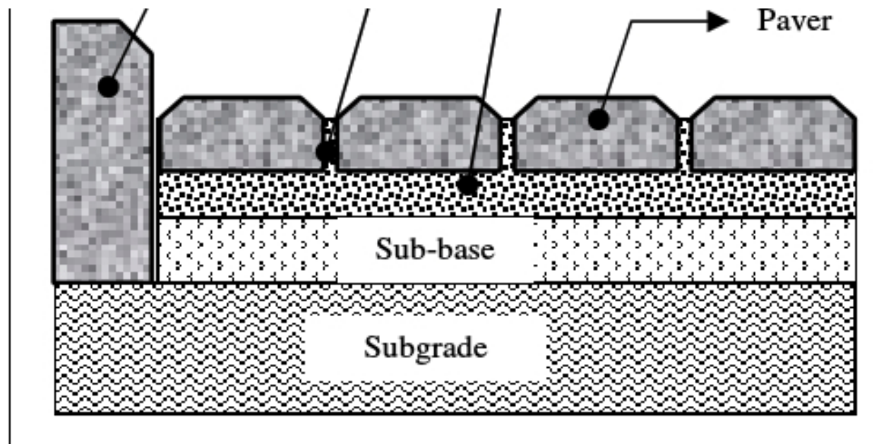
Figure 1. Structure of concrete block pavement
