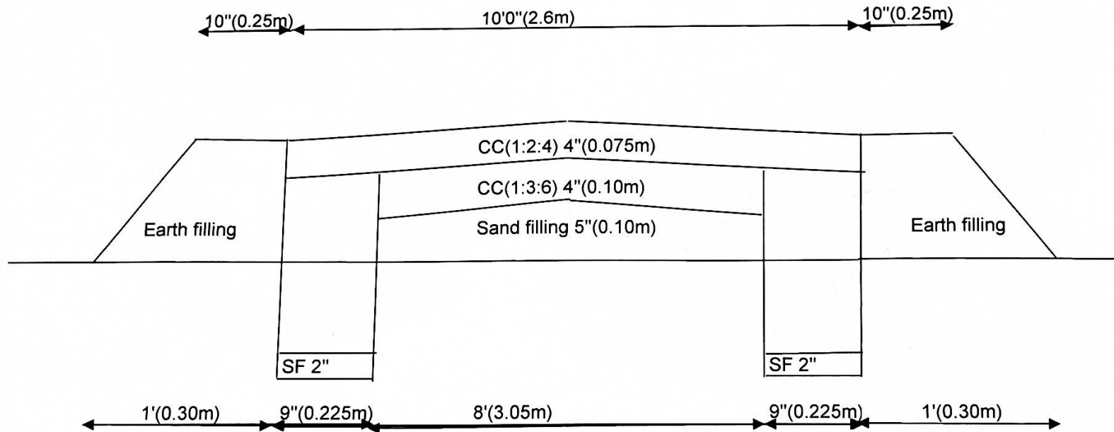
CROSS SECTION OF ROAD (NTS)
