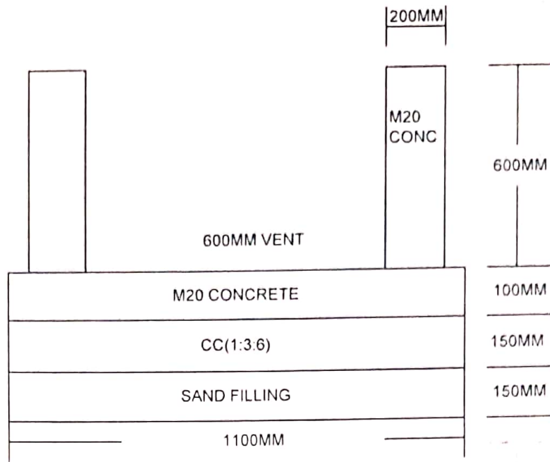
SECTIONAL ELEVATION
