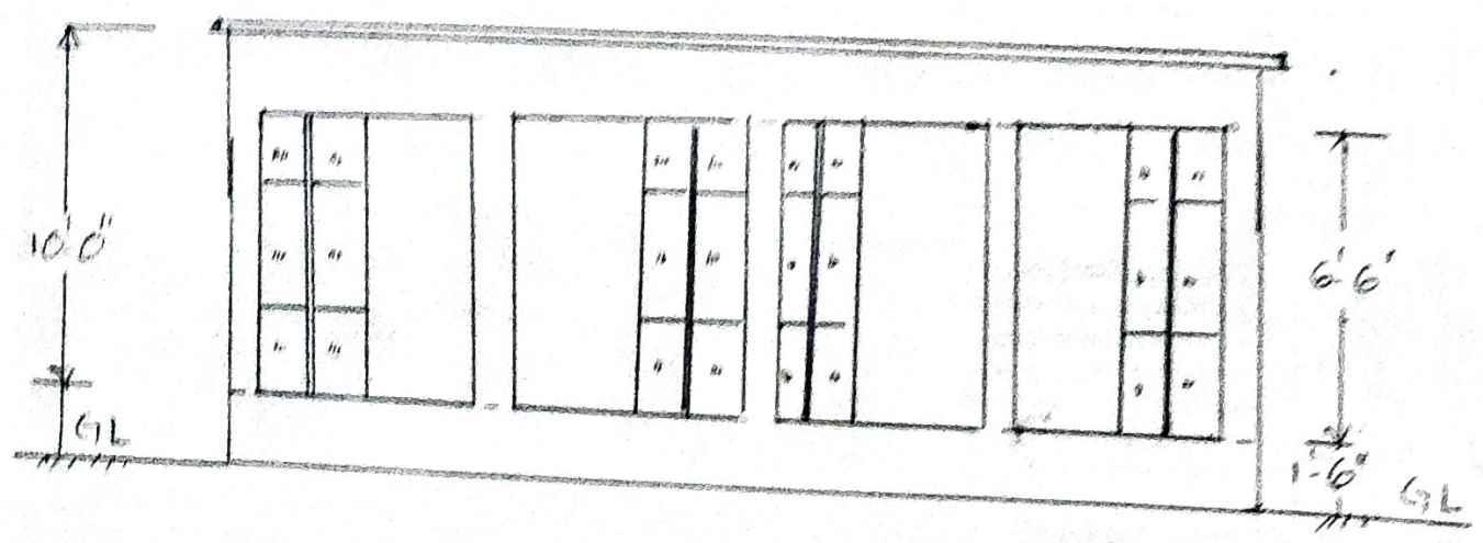
ELEVATION.
