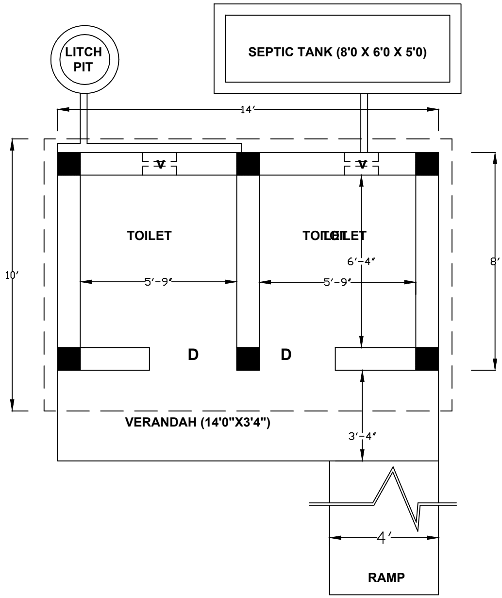
DETAIL PLAN OF GIRL'S TOILET UNDER SSA FOR THE F.Y. 2022-23
