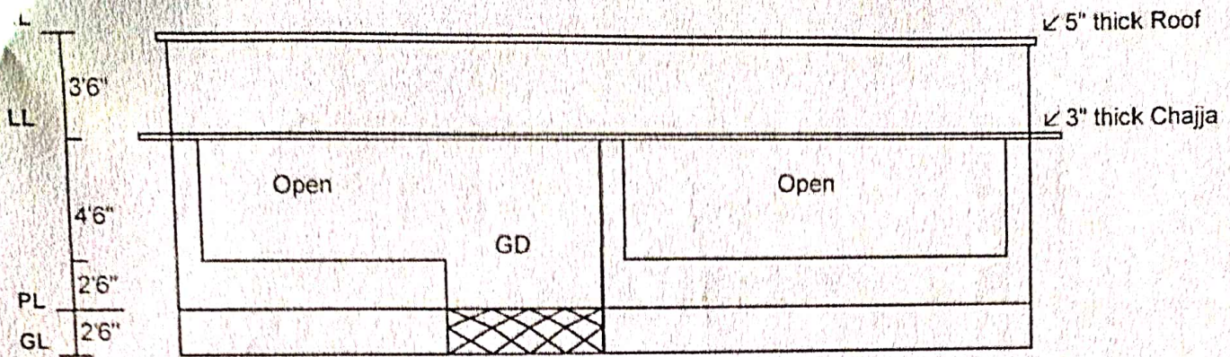
Front Sectional Elevation
