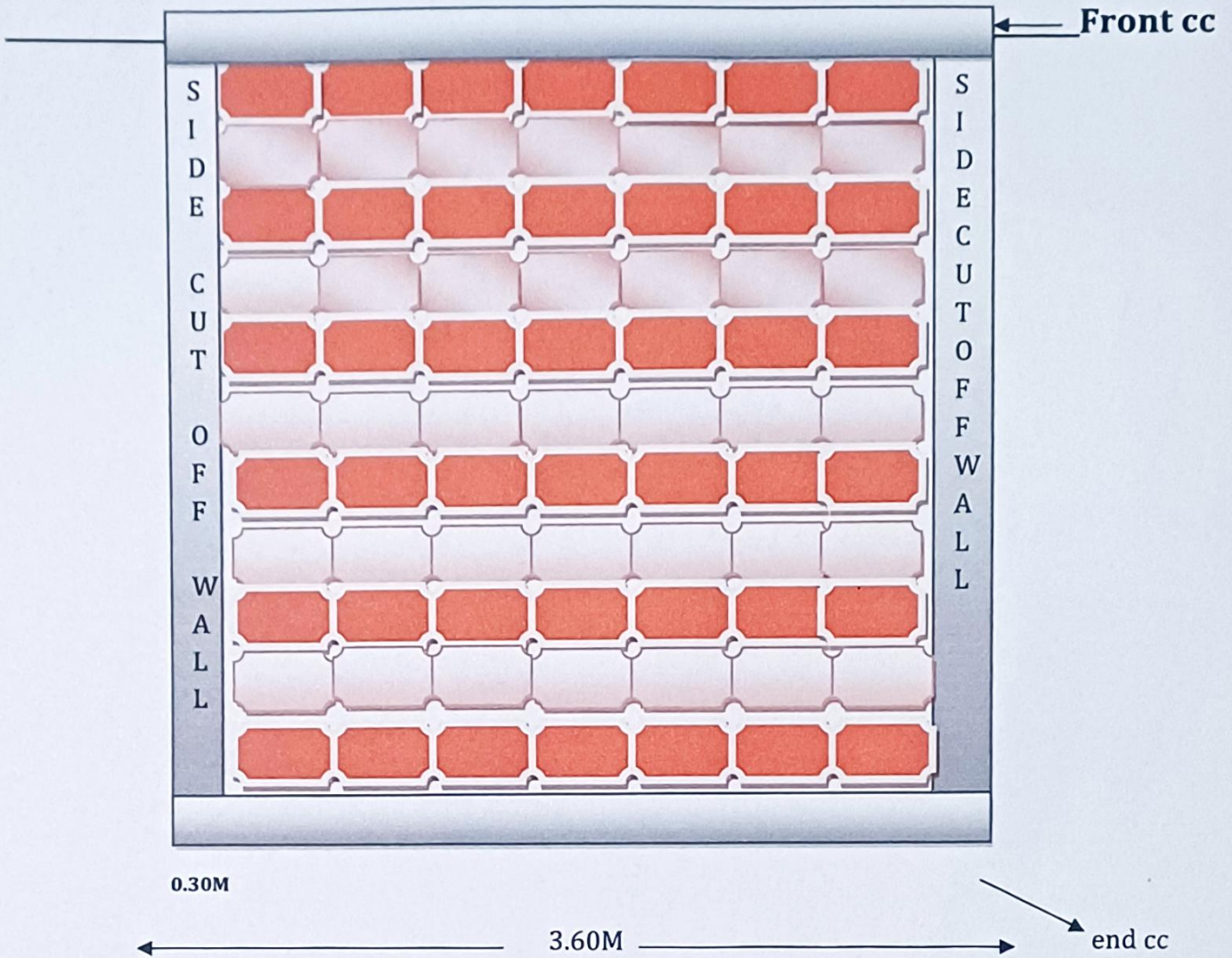
PAVER BLOCK DRAWING
