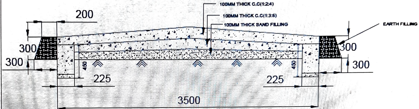
CROSS SECTION OF CEMENT CONCRETE ROAD WITH CUT OFF WALL
