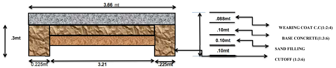
CROSS SECTION OF CC ROAD
