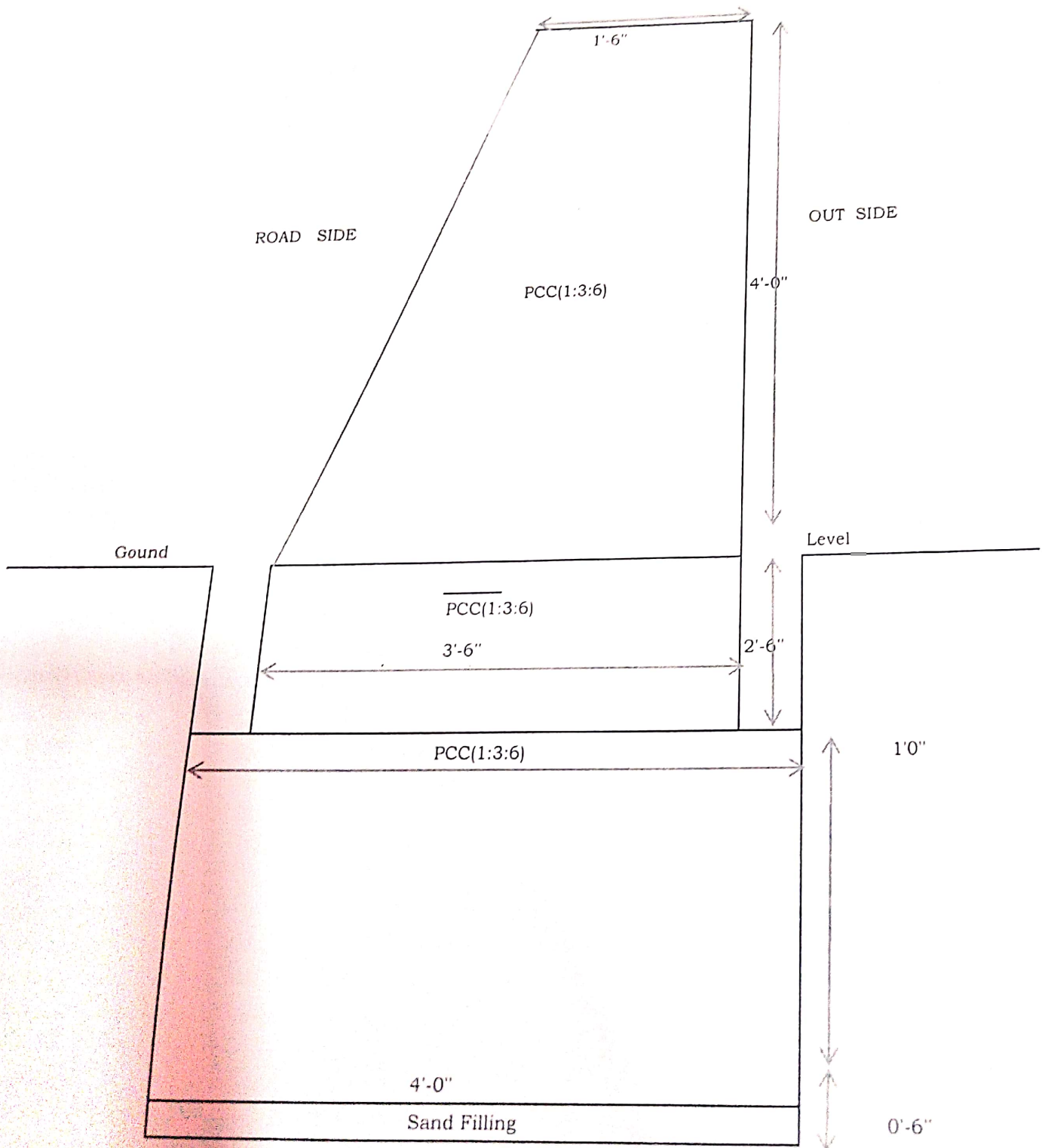
Typical cross section of Guard wall
