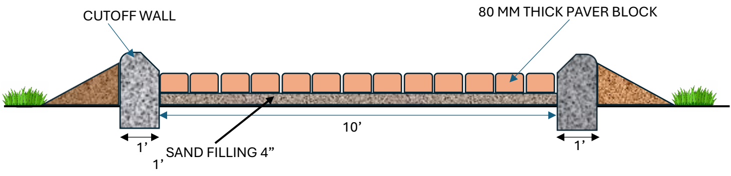
CROSS SECTION OF A TYPICAL PAVER ROAD SECTION
