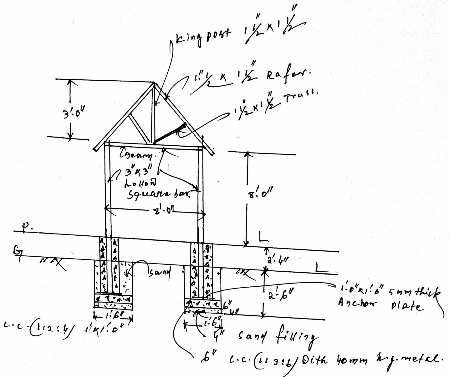
SECTION OF HATT PINDI
