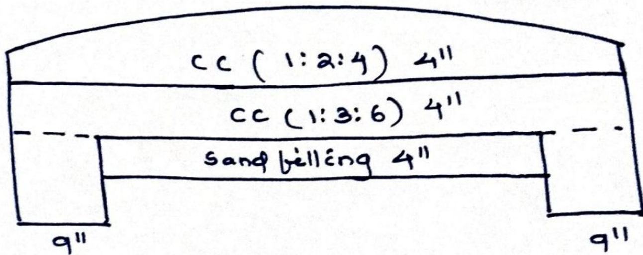
Cement Concrete Road. (Drawing)
