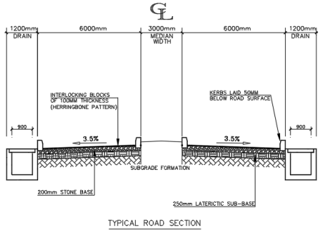
TYPICAL ROAD SECTION
