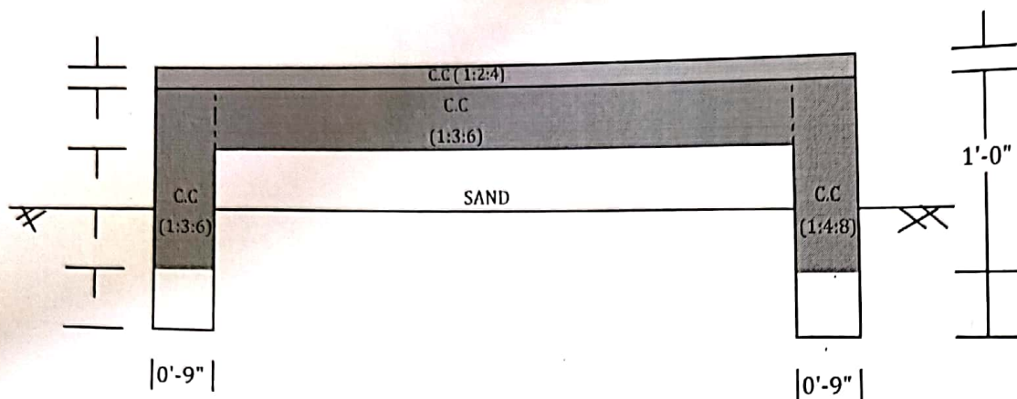
SECTION OF C.C ROAD
