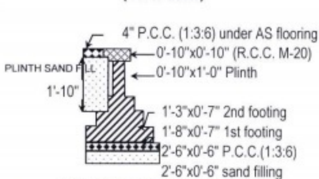
FOUNDATION SECTION OF WALL
