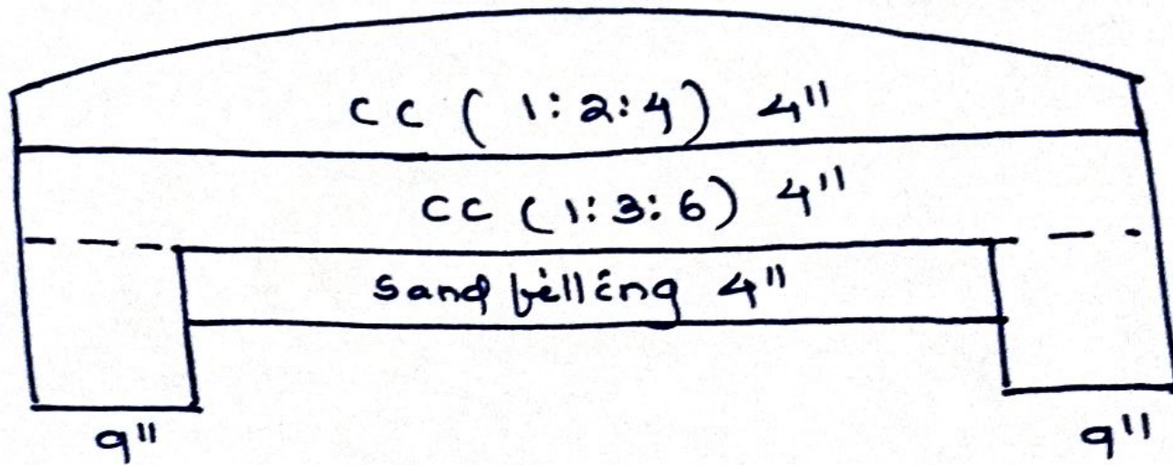
Cement Concrete Road. (Drawing)
