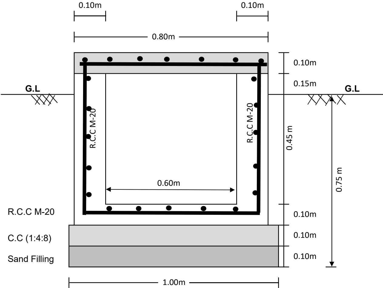
CROSS SECTION OF R.C.C DRAIN
