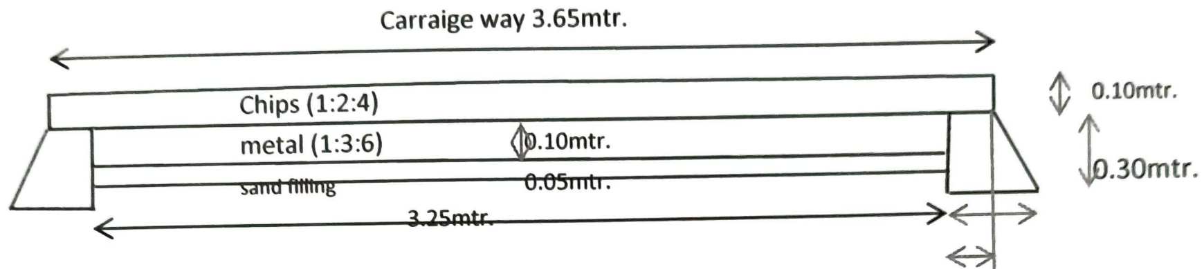
CROSSECTION OF THE CEMENT CONCRETE ROAD
