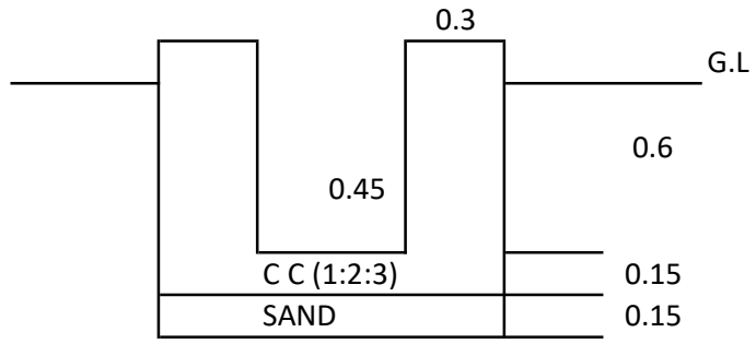
1.05 CEMENT CONCRETE DRAIN
