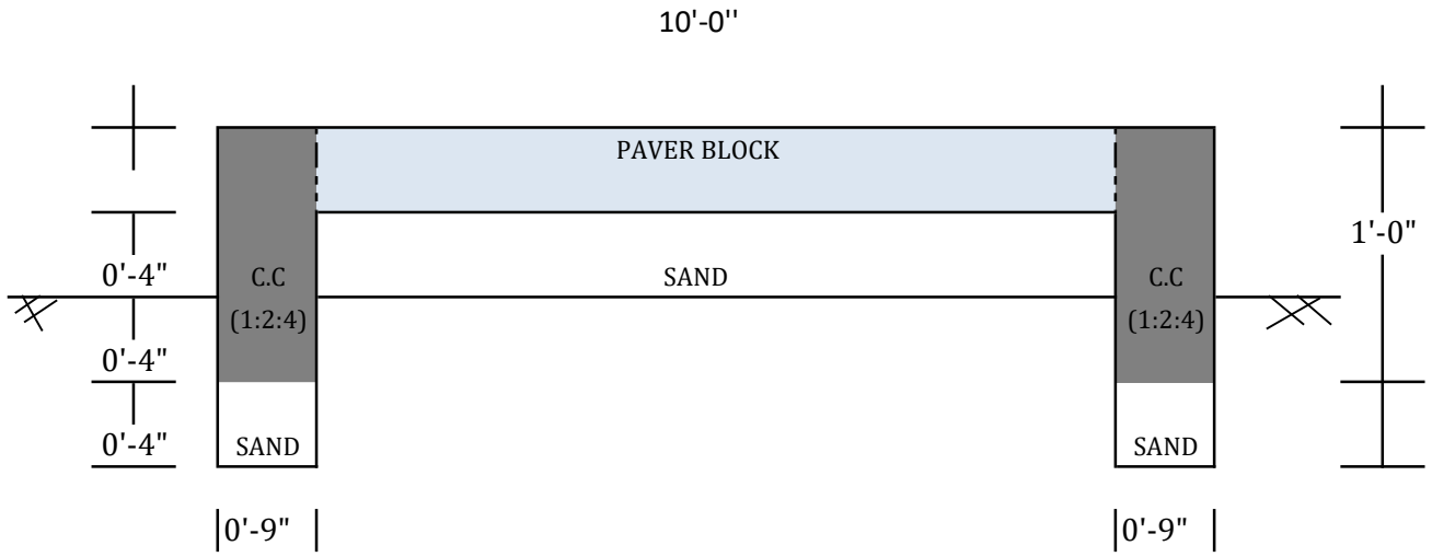
SECTION OF PAVER BLOCK ROAD
