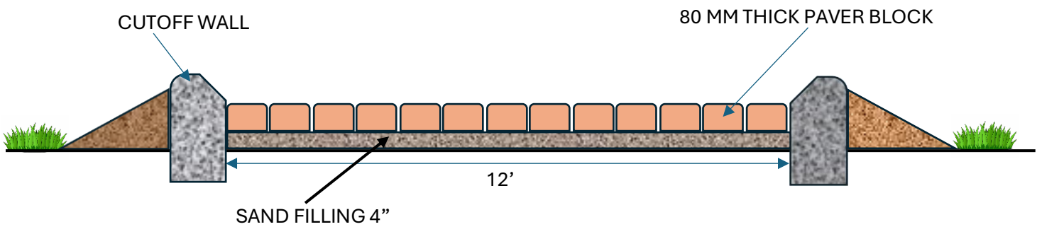
CROSS SECTION OF A TYPICAL PAVER ROAD SECTION
