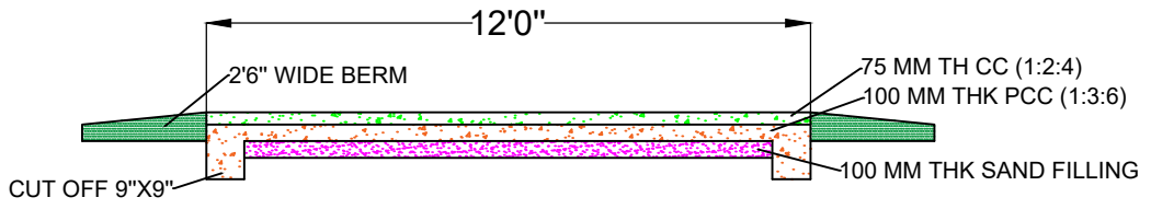
C/S ELEVATION OF ROAD
