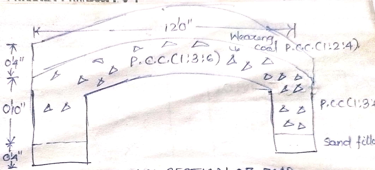
CROSS SECTION OF ROAD.
