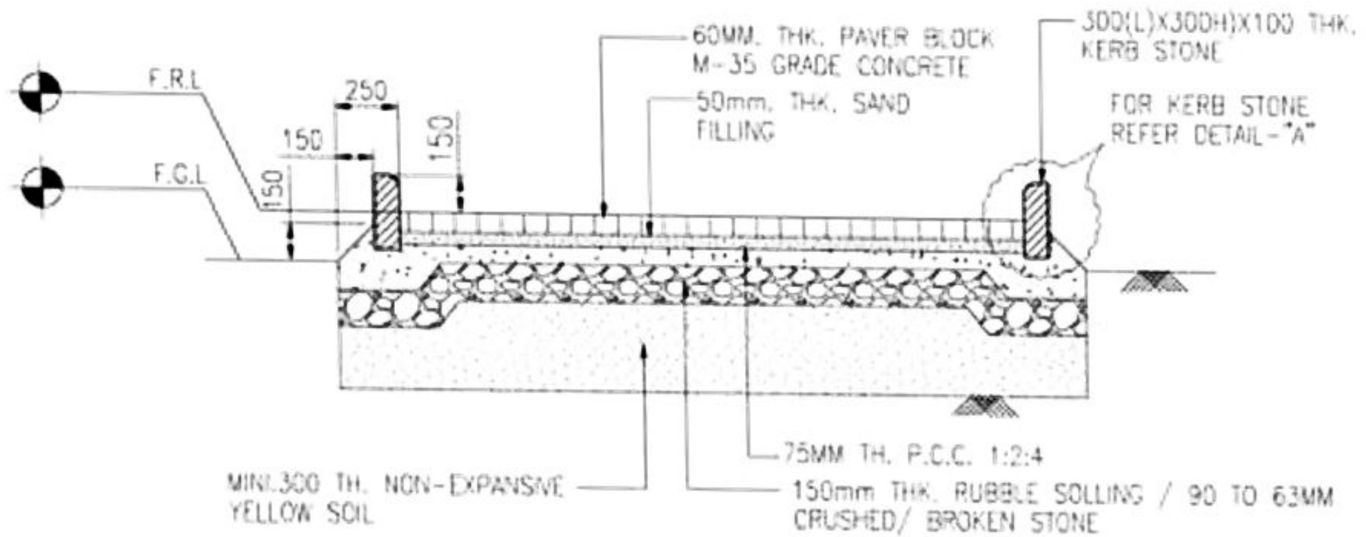
TYPICAL SECTION FOR PAVER BLOCK
