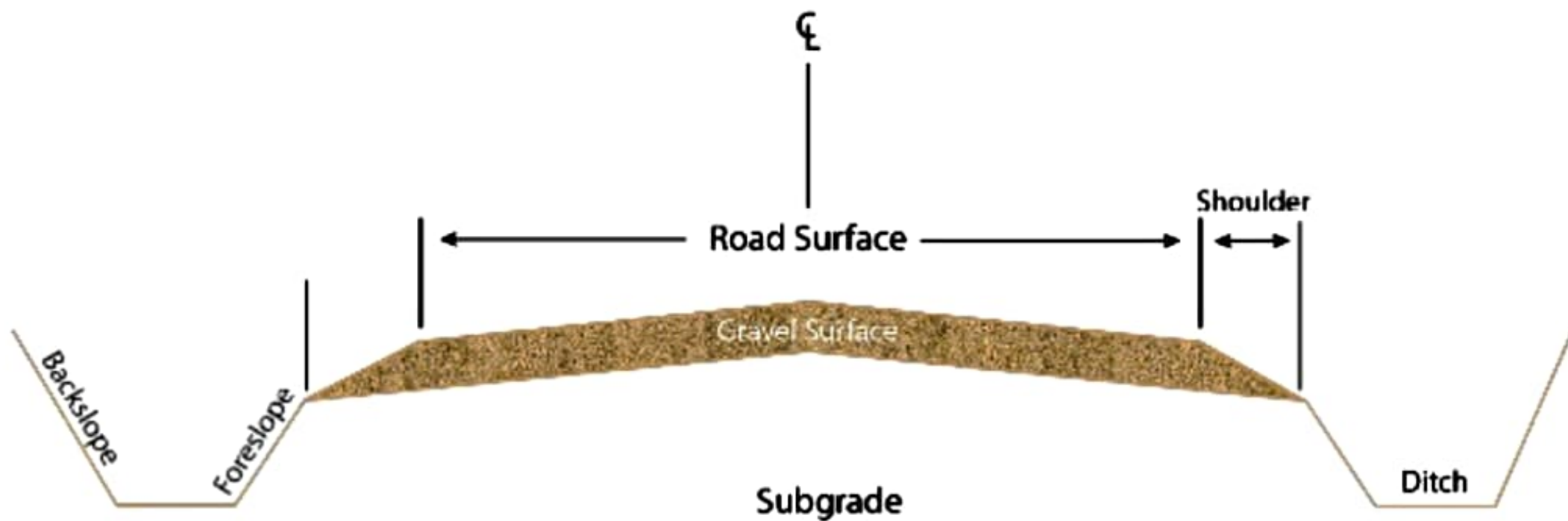
Figure 1: The components of the roadway cross section.
