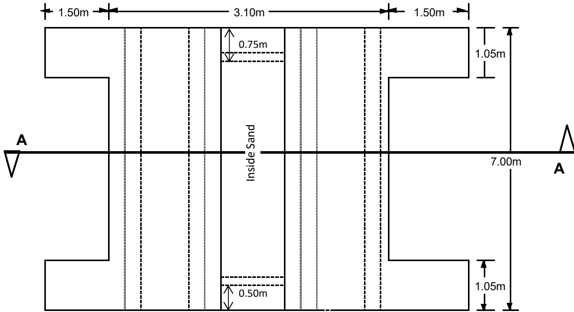
PLAN OF CULVERT
