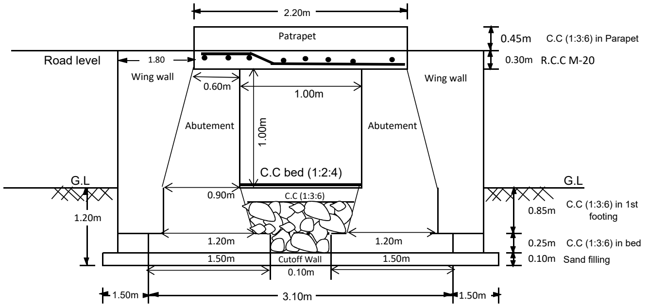
CROSS SECTION OF CULVERT
