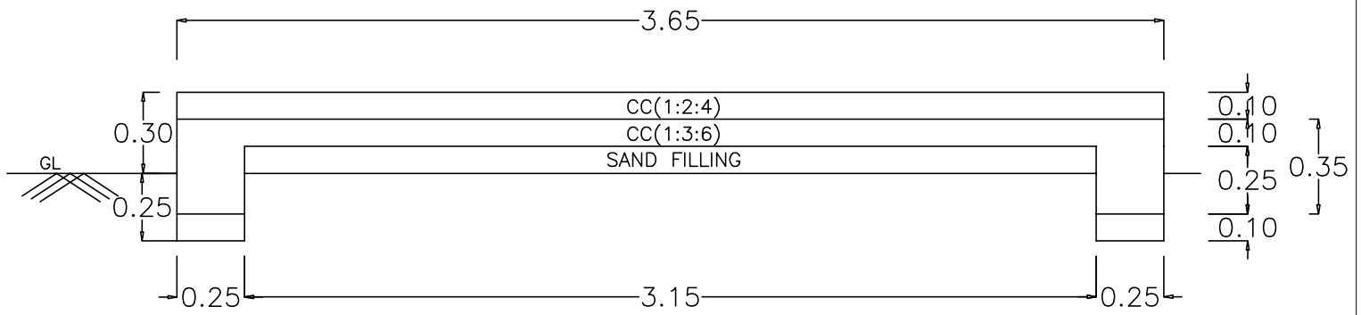
CROSS-SECTION OF CC ROAD
